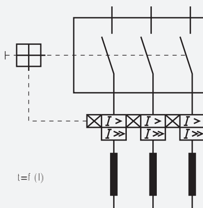
Three Pole Schematic Diagram
